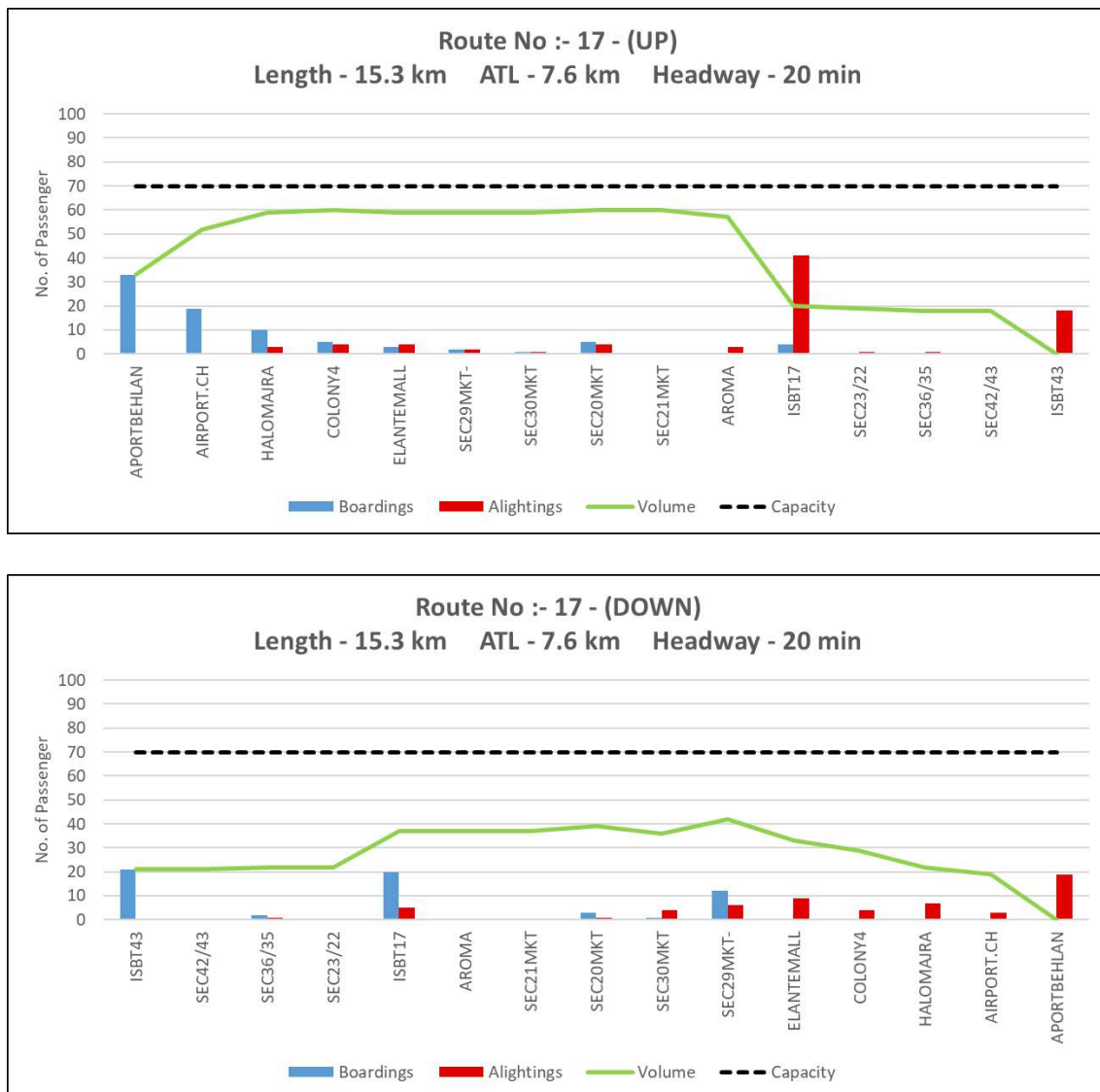
Figure 3: Peak hour Boarding & Alighting pattern along with line load of Route 17 (Up and Down)
