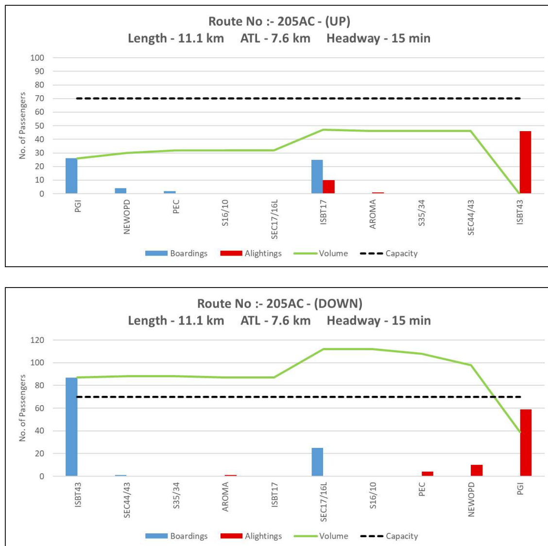
Figure 23: Peak hour Boarding & Alighting pattern along with line load of Route 205AC (Up and Down)
