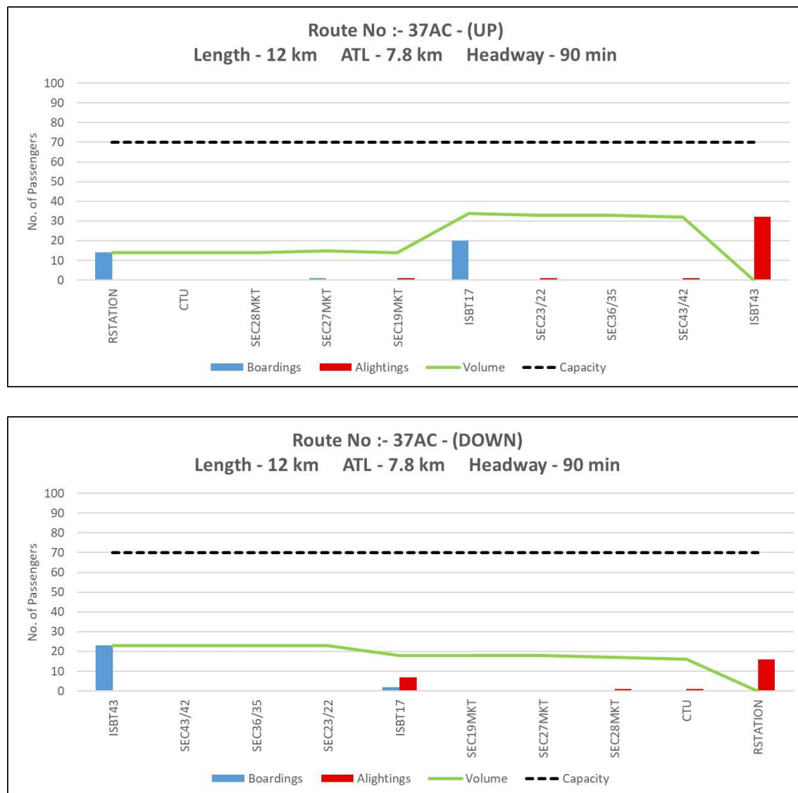
Figure 20: Peak hour Boarding & Alighting pattern along with line load of Route 37AC (Up and Down)
