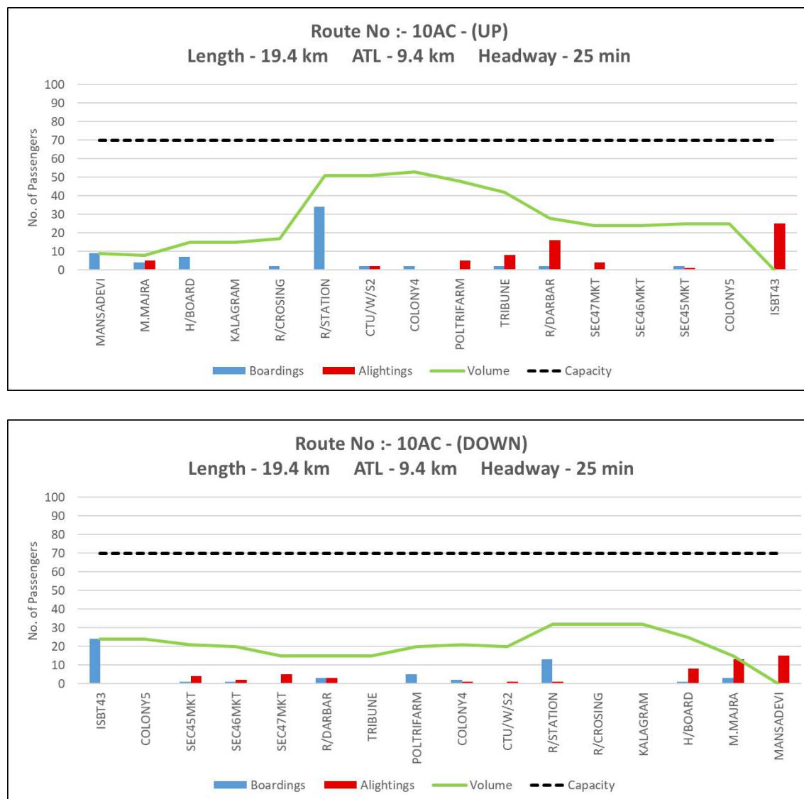
Figure 19: Peak hour Boarding & Alighting pattern along with line load of Route 10AC (Up and Down)
