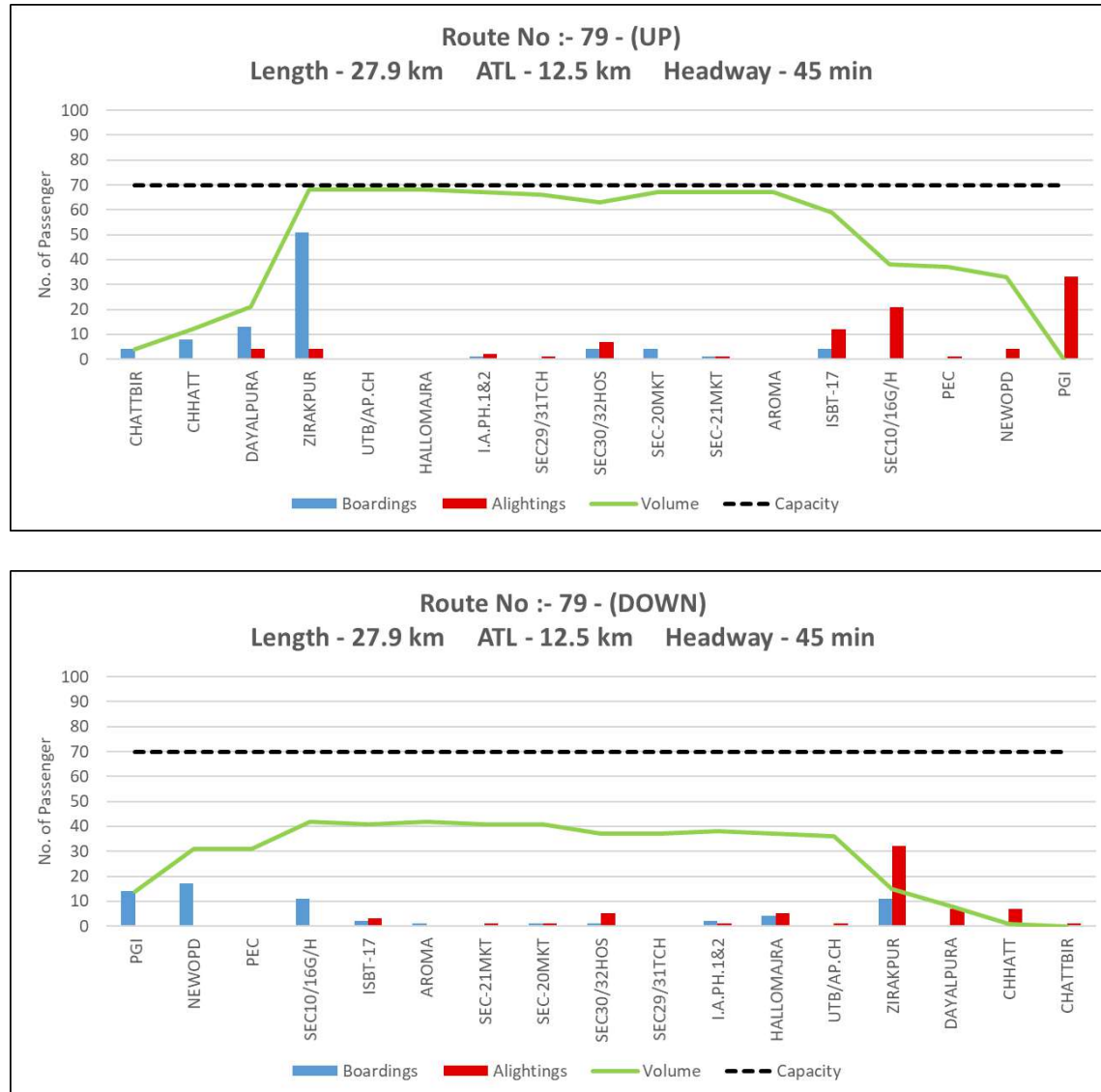
Figure 37: Peak hour Boarding & Alighting pattern along with line load of Route 79 (Up and Down)
