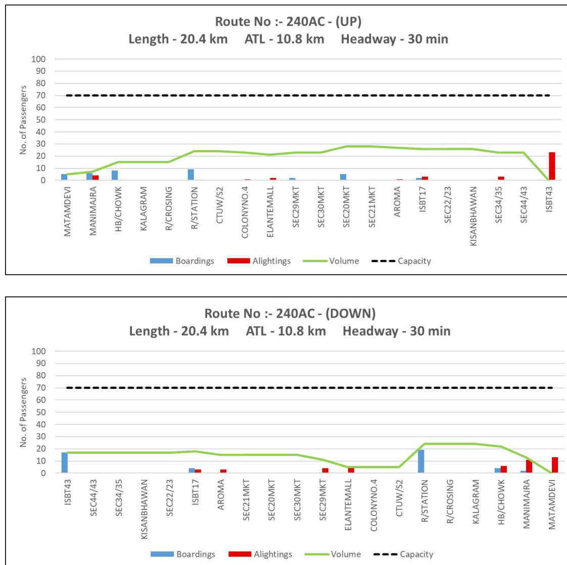
Figure 25: Peak hour Boarding & Alighting pattern along with line load of Route 240AC (Up and Down)
