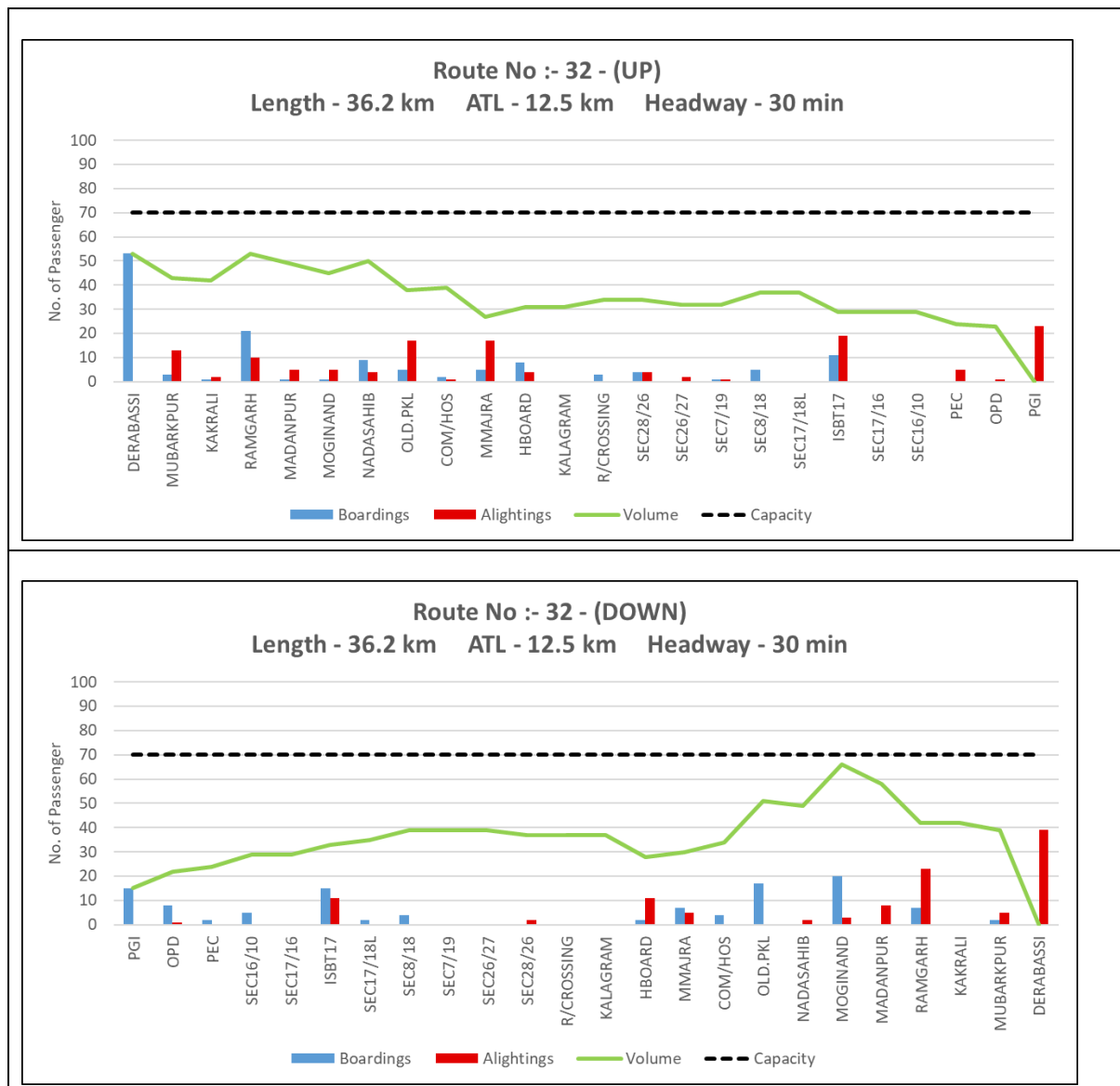
Figure 32: Peak hour Boarding & Alighting pattern along with line load of Route 32 (Up and Down)
