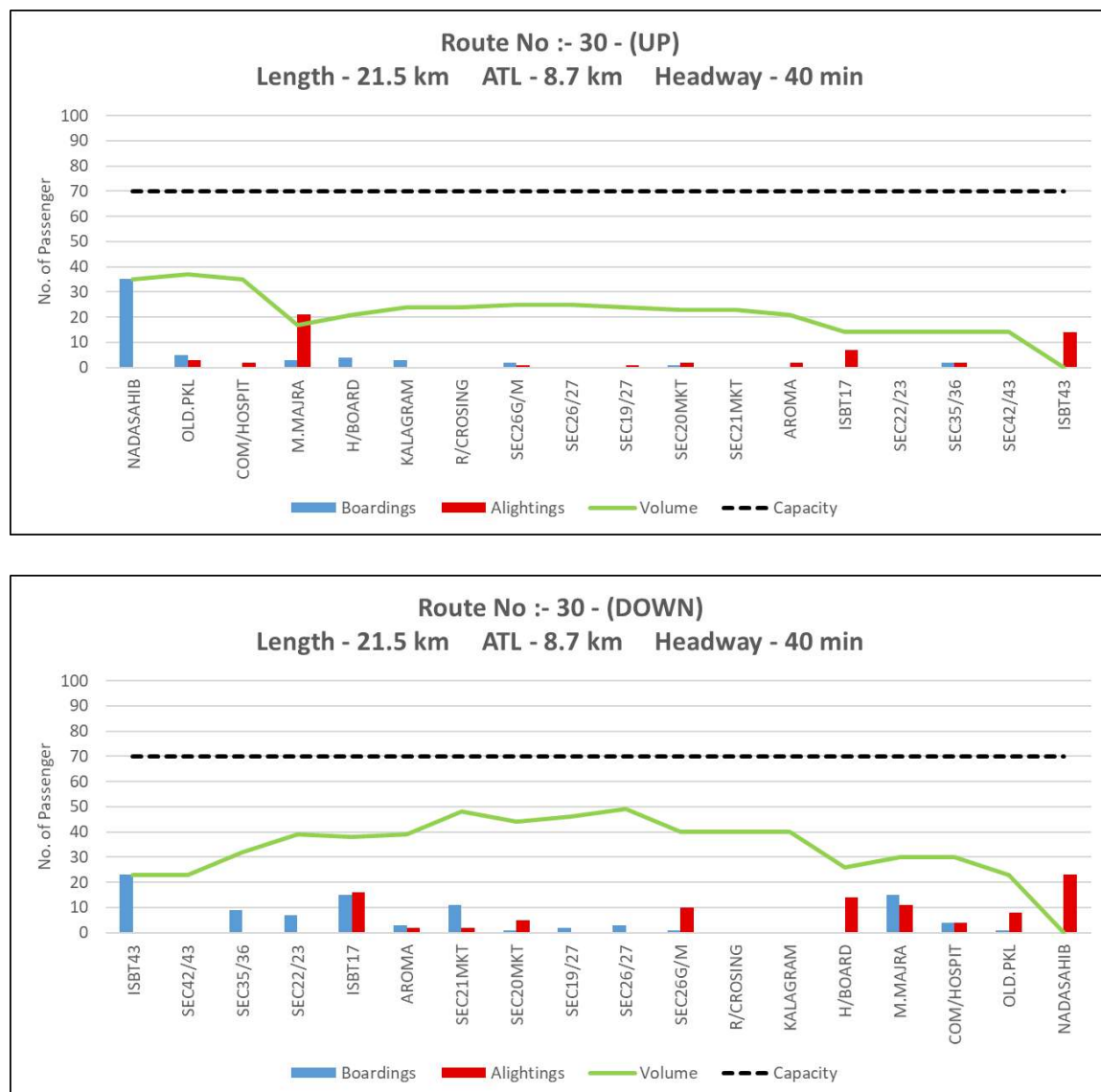
Figure 31: Peak hour Boarding & Alighting pattern along with line load of Route 30 (Up and Down)
