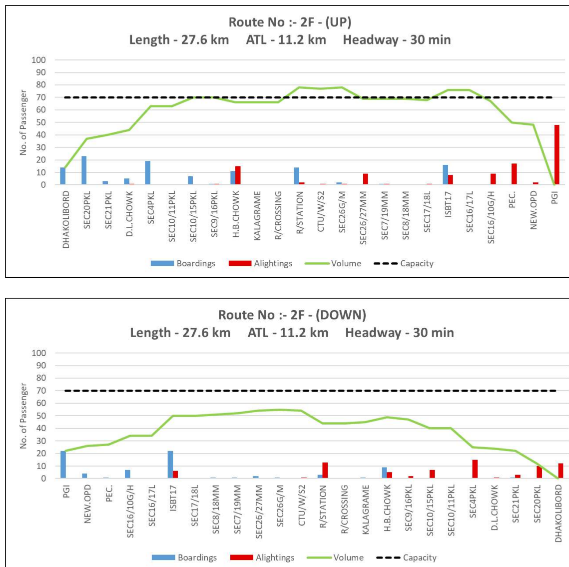
Figure 43: Peak hour Boarding & Alighting pattern along with line load of Route 2F (Up and Down)
