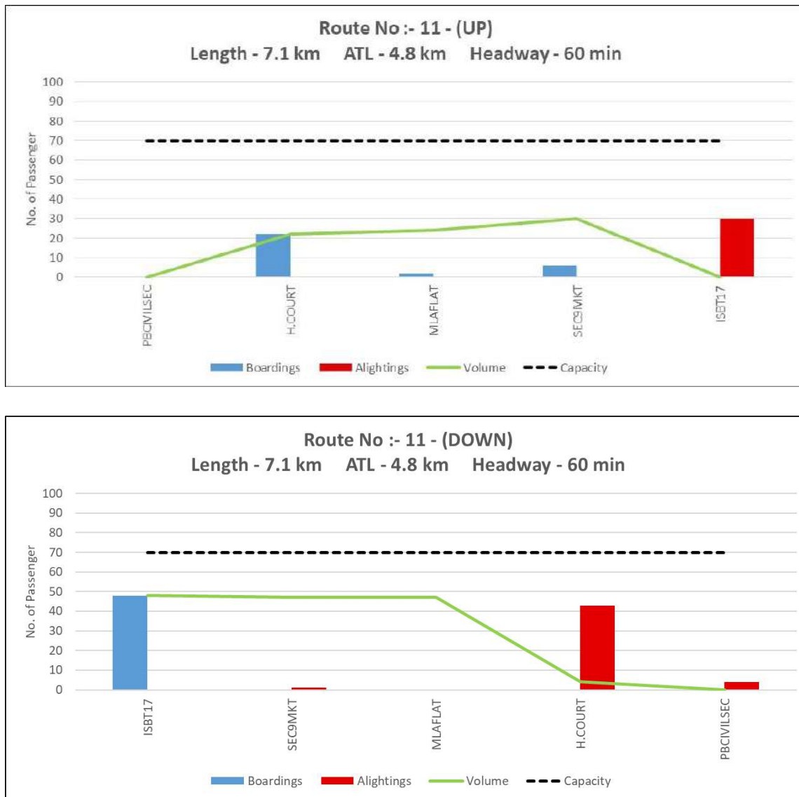
Figure 2: Peak hour Boarding & Alighting pattern along with line load of Route 11 (Up and Down)
