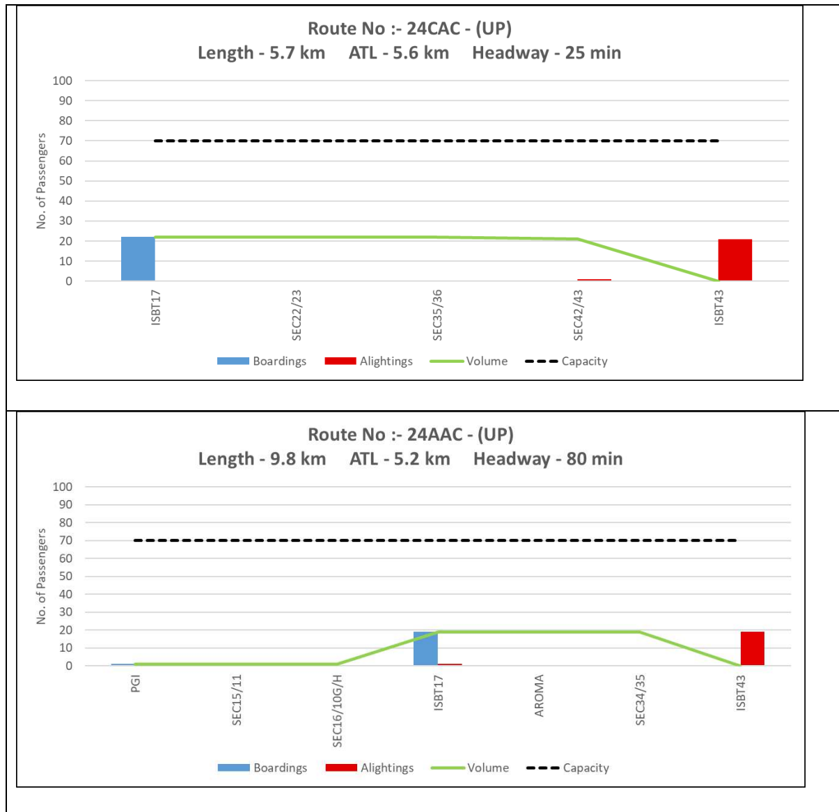
Figure 26: Peak hour Boarding & Alighting pattern along with line load of Route 24AAC and 24CAC
