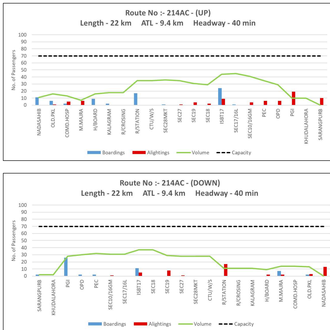
Figure 57: Peak hour Boarding & Alighting pattern along with line load of Route 214AC (Up and Down)
