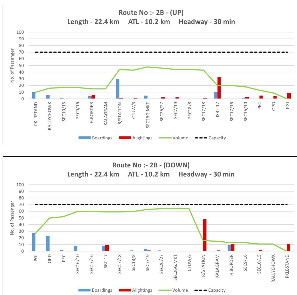
Figure 42: Peak hour Boarding & Alighting pattern along with line load of Route 2B (Up and Down)
