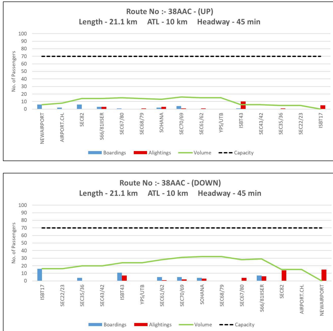
Figure 59: Peak hour Boarding & Alighting pattern along with line load of Route 38AAC (Up and Down)
