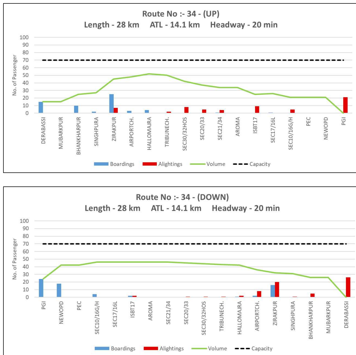
Figure 33: Peak hour Boarding & Alighting pattern along with line load of Route 34 (Up and Down)
