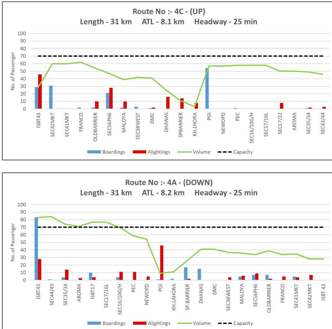
Figure 13: Peak hour Boarding & Alighting pattern along with line load of Route 4A and 4C
