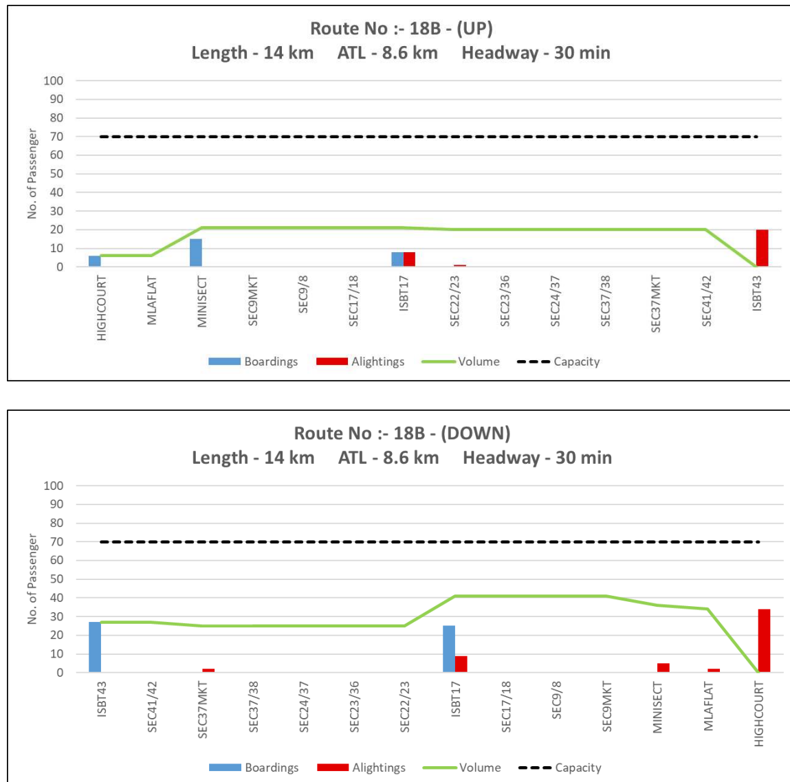
Figure 16: Peak hour Boarding & Alighting pattern along with line load of Route 18B (Up and Down)
