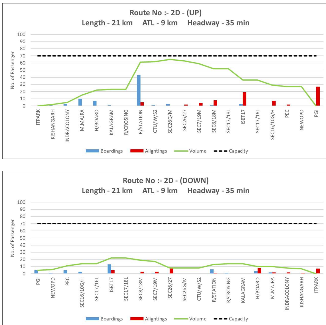
Figure 12: Peak hour Boarding & Alighting pattern along with line load of Route 2D (Up and Down)
