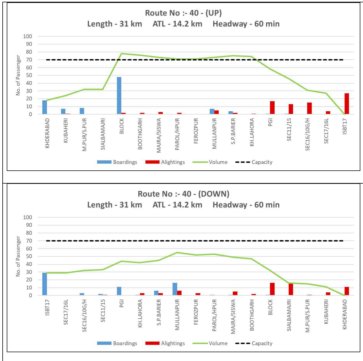
Figure 36: Peak hour Boarding & Alighting pattern along with line load of Route 40 (Up and Down)
