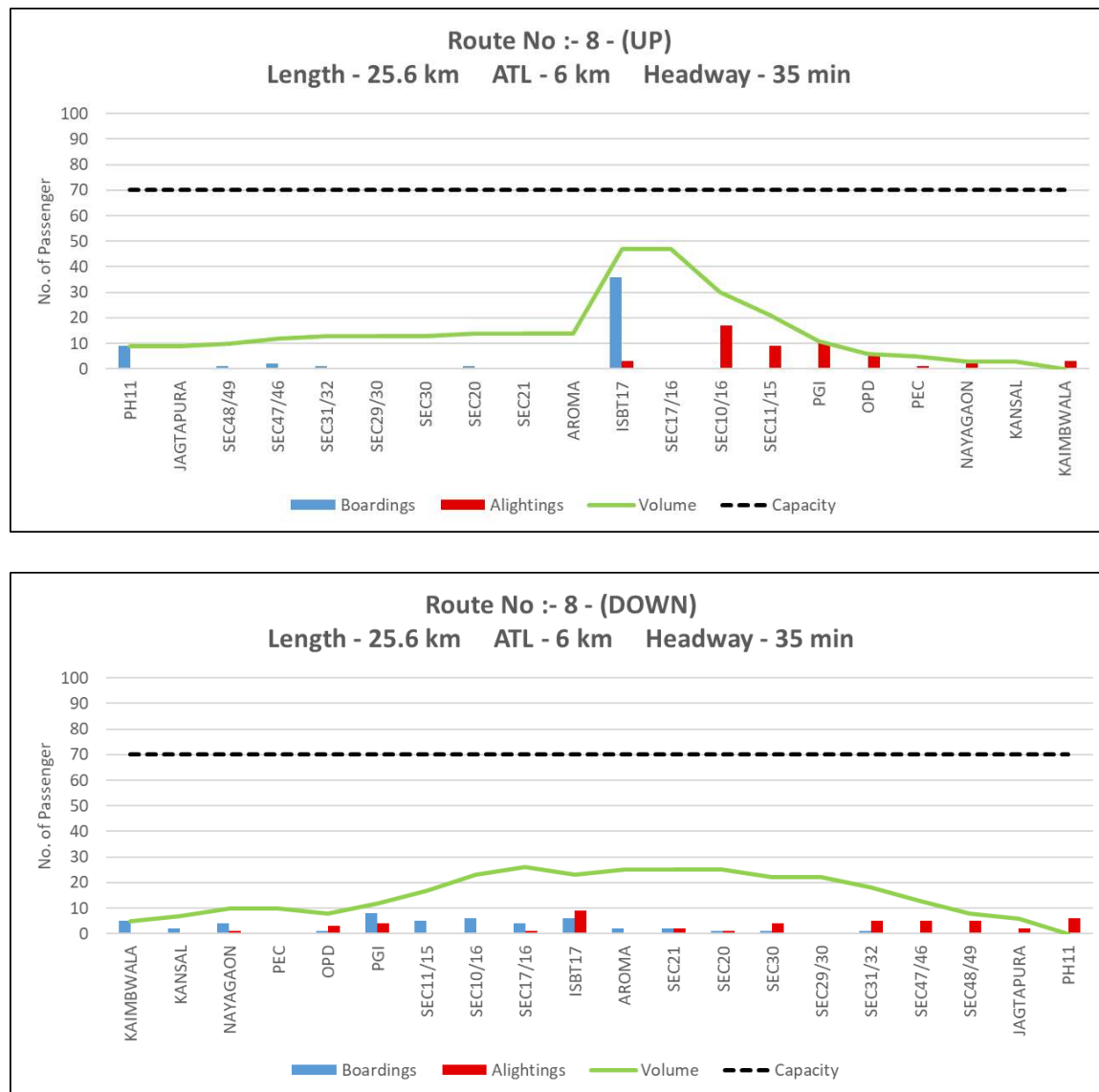
Figure 29: Peak hour Boarding & Alighting pattern along with line load of Route 8 (Up and Down)
