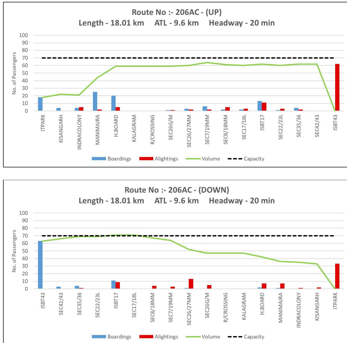
Figure 24: Peak hour Boarding & Alighting pattern along with line load of Route 206AC (Up and Down)
