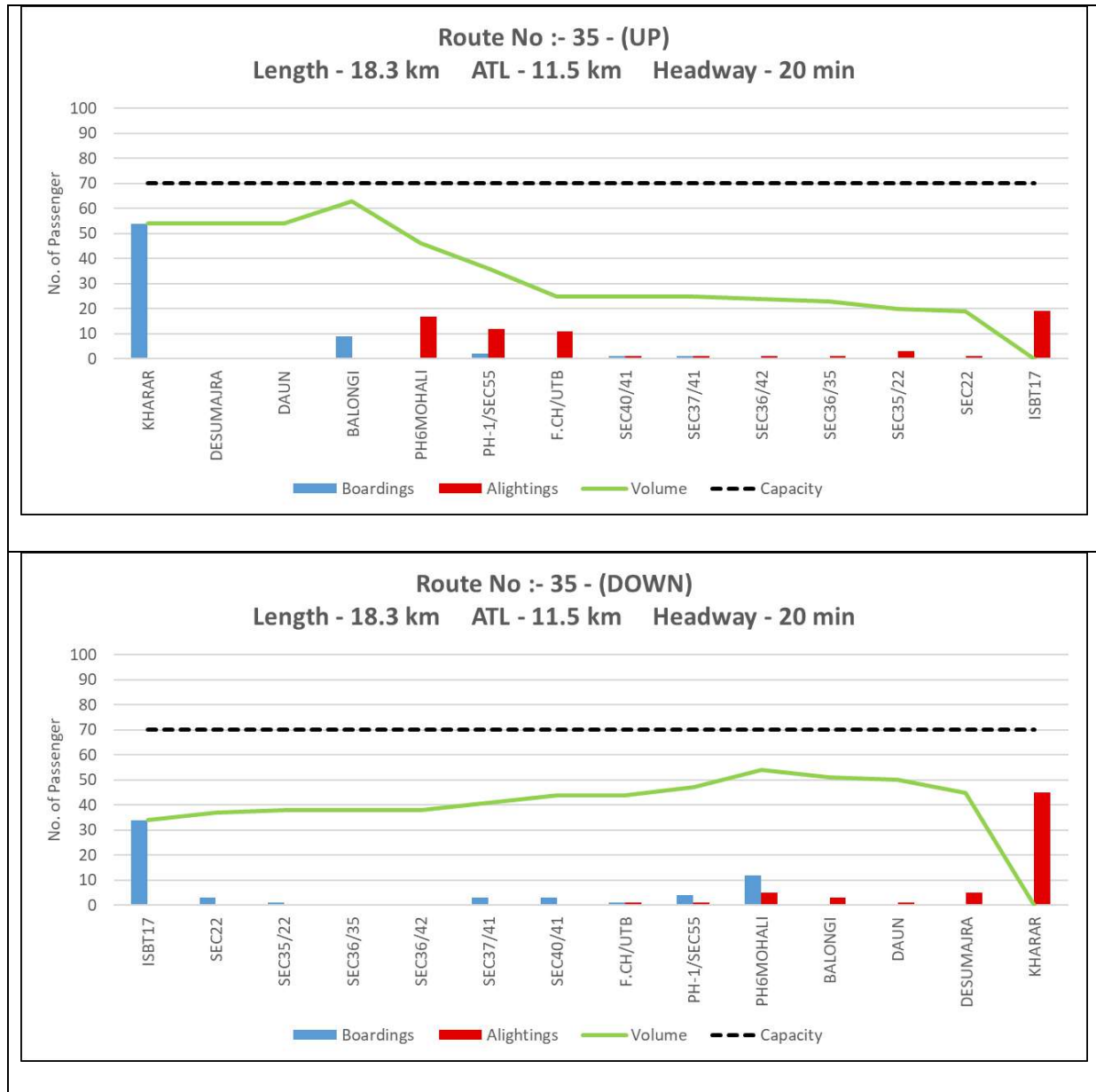
Figure 34: Peak hour Boarding & Alighting pattern along with line load of Route 35 (Up and Down)
