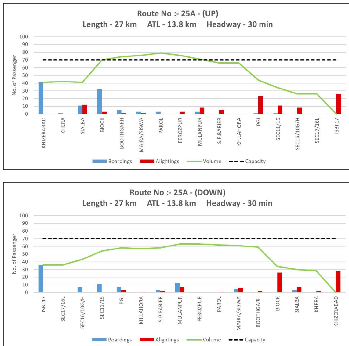
Figure 46: Peak hour Boarding & Alighting pattern along with line load of Route 25A
