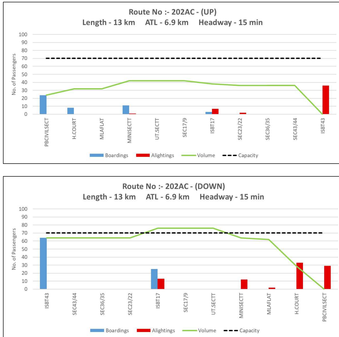
Figure 21: Peak hour Boarding & Alighting pattern along with line load of Route 202AC (Up and Down)
