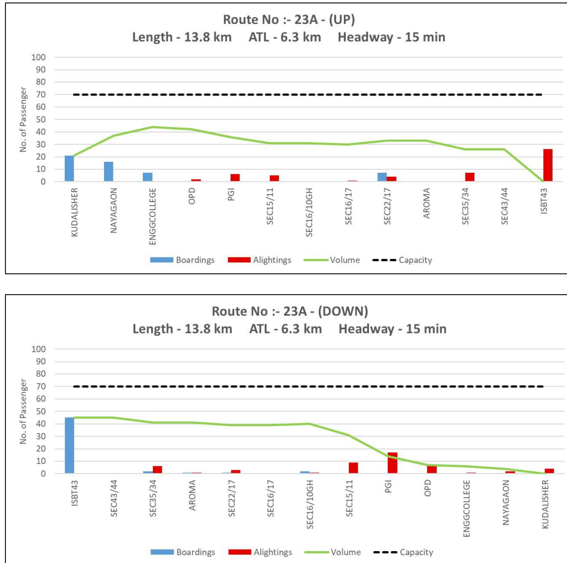
Figure 17: Peak hour Boarding & Alighting pattern along with line load of Route 23A (Up and Down)
