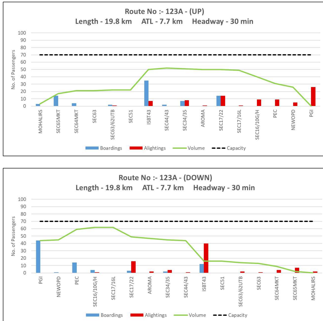
Figure 51: Peak hour Boarding & Alighting pattern along with line load of Route 123A (Up and Down)
