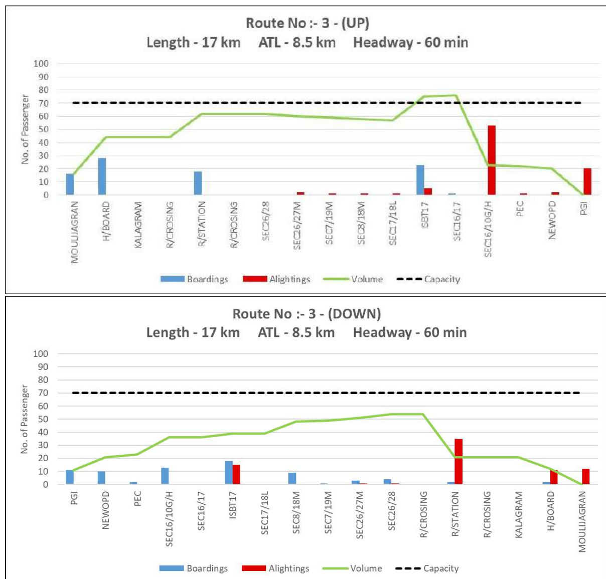
Figure 1: Peak hour Boarding & Alighting pattern along with line load of Route 3 (Up and Down)
