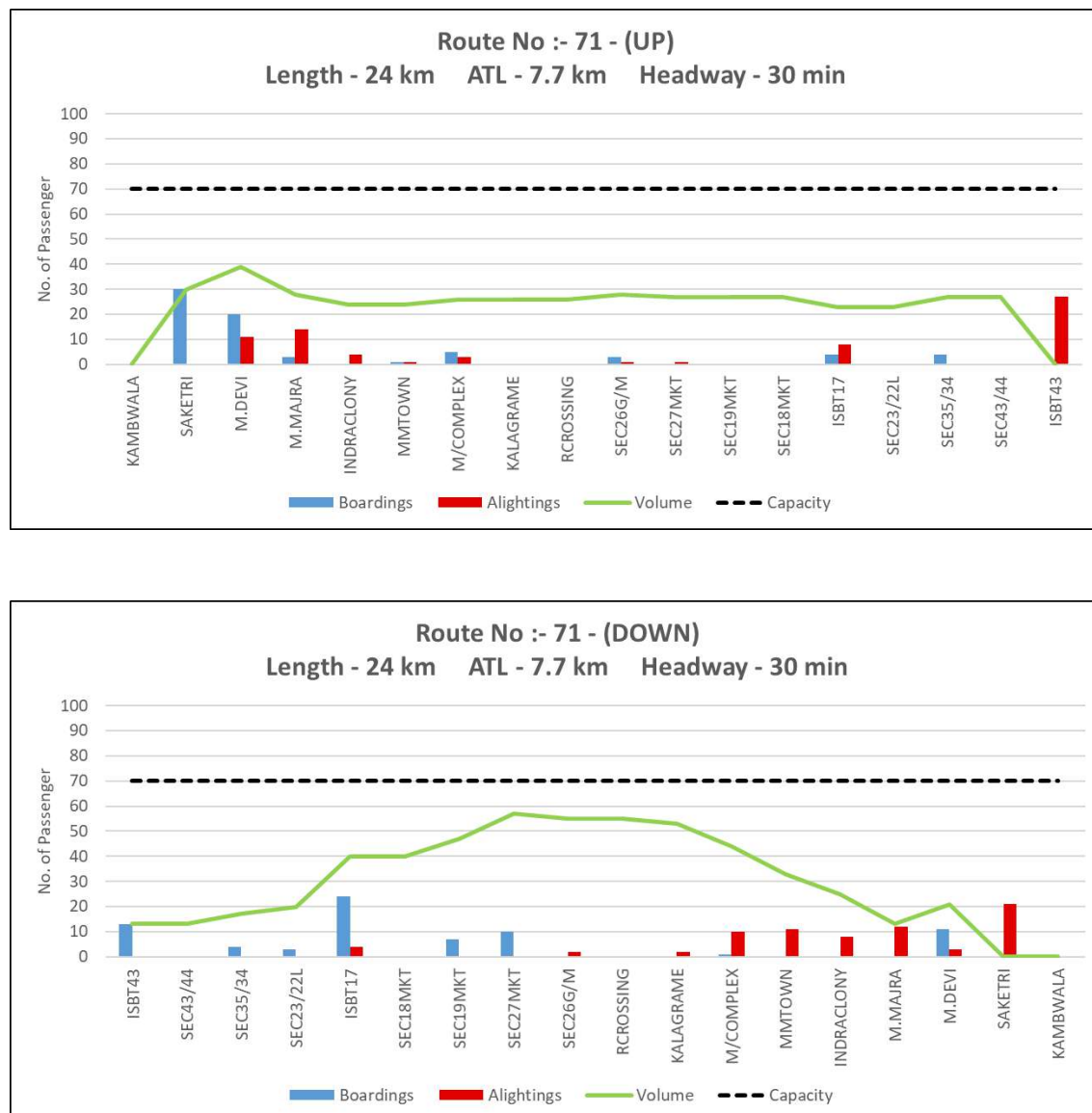
Figure 7: Peak hour Boarding & Alighting pattern along with line load of Route 71 (Up and Down)
