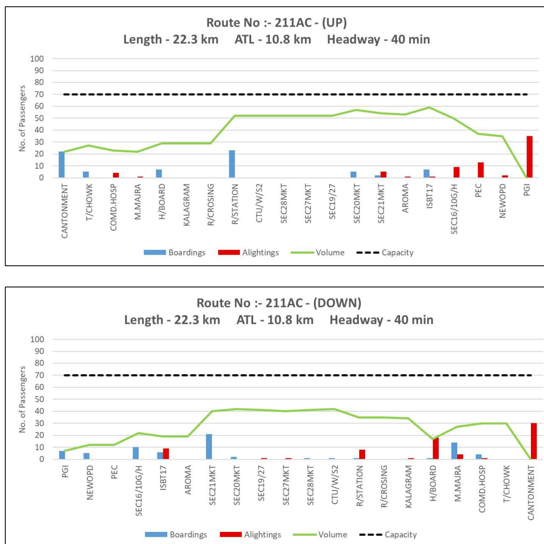
Figure 56: Peak hour Boarding & Alighting pattern along with line load of Route 211AC (Up and Down)
