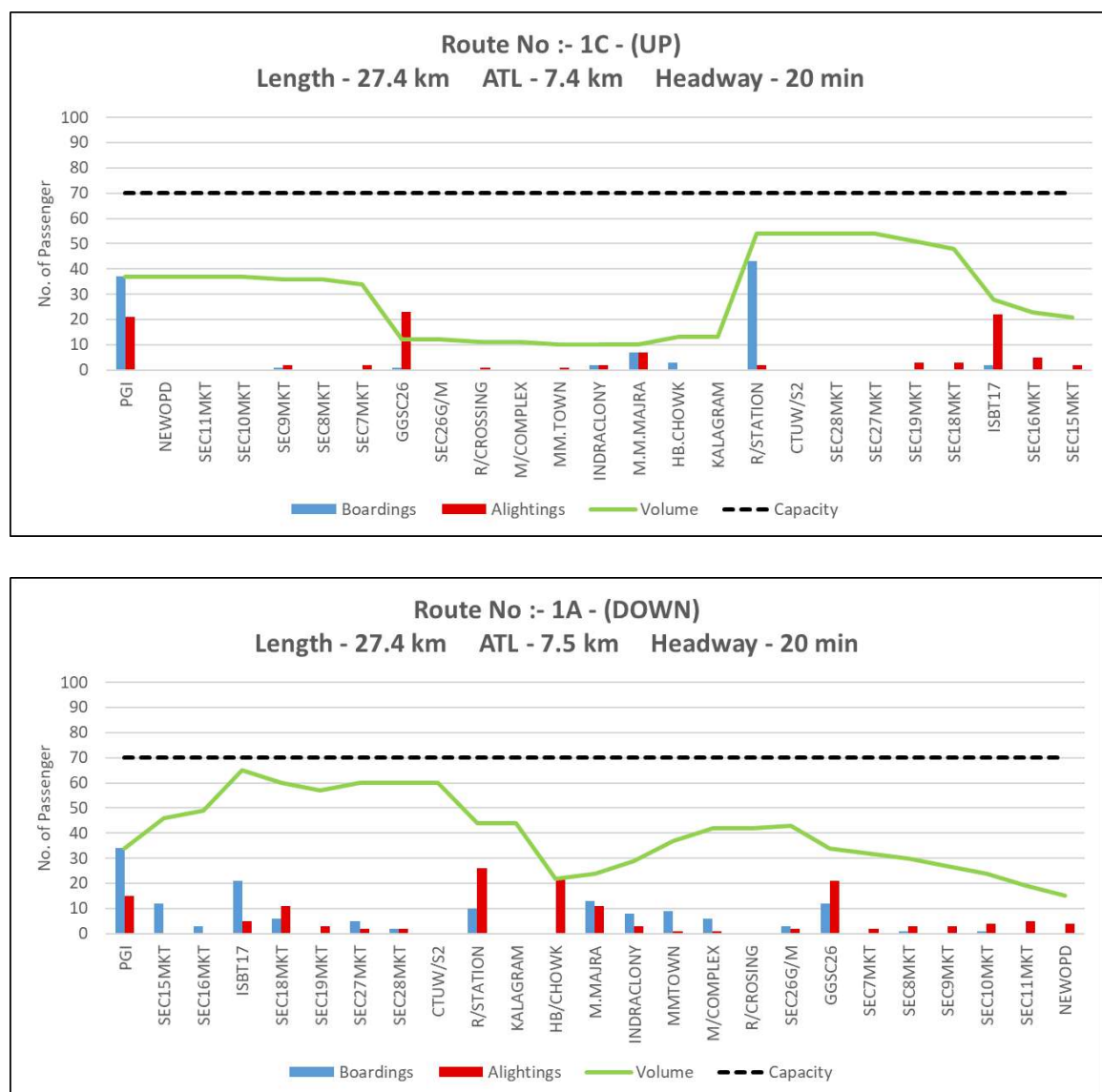
Figure 10: Peak hour Boarding & Alighting pattern along with line load of Route 1A and 1C
