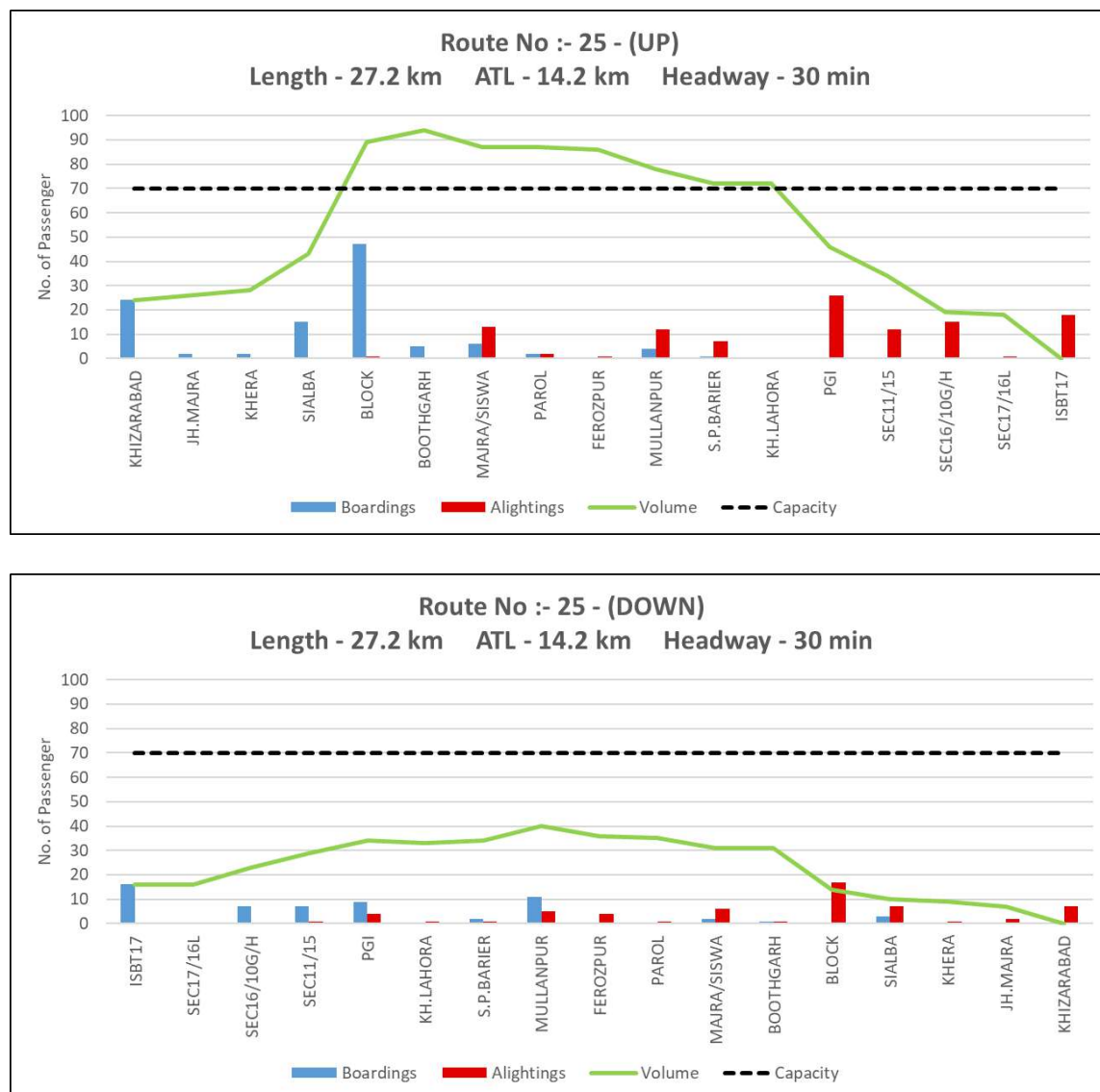
Figure 30: Peak hour Boarding & Alighting pattern along with line load of Route 25 (Up and Down)
