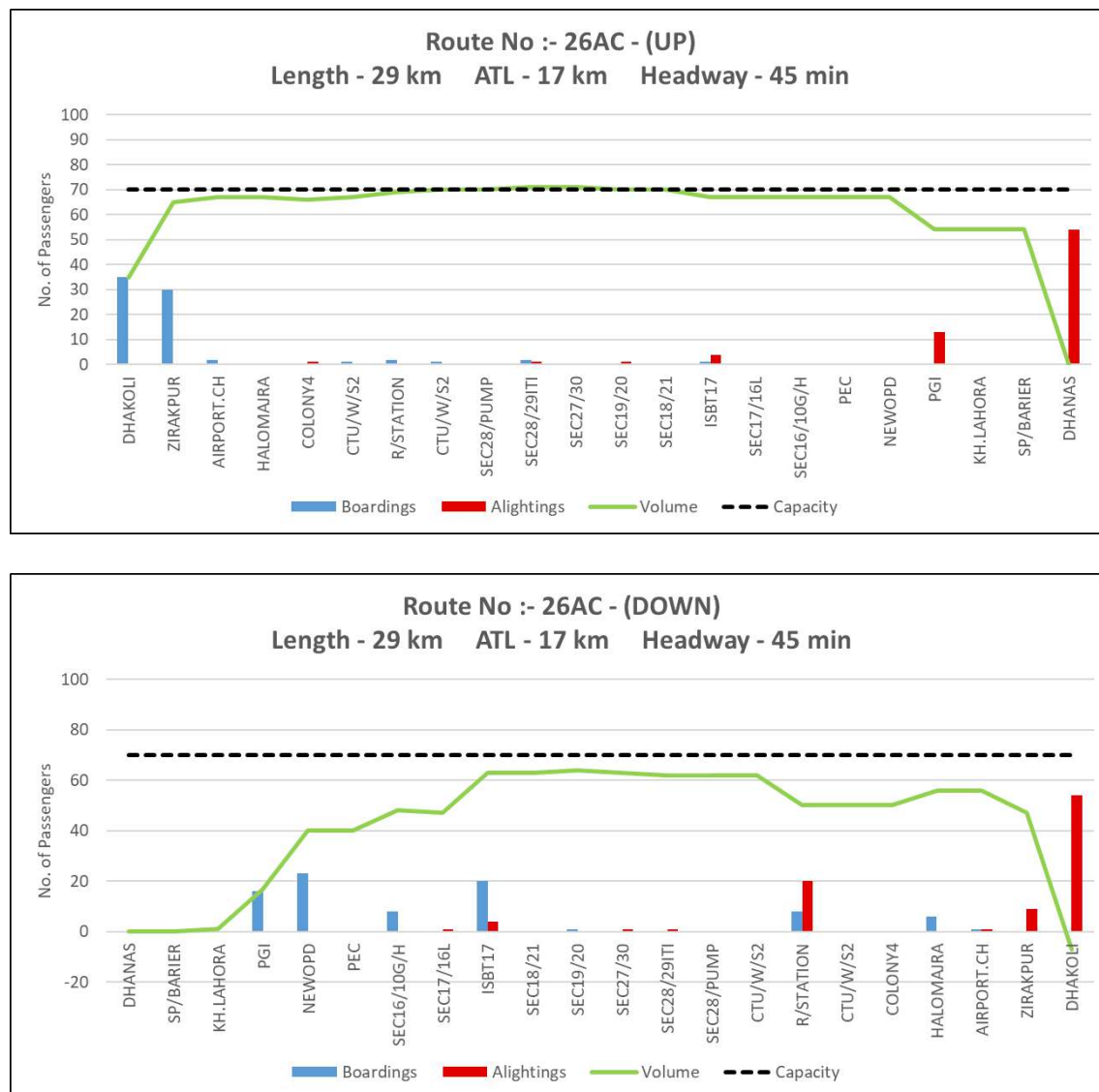
Figure 53: Peak hour Boarding & Alighting pattern along with line load of Route 26AC (Up and Down)
