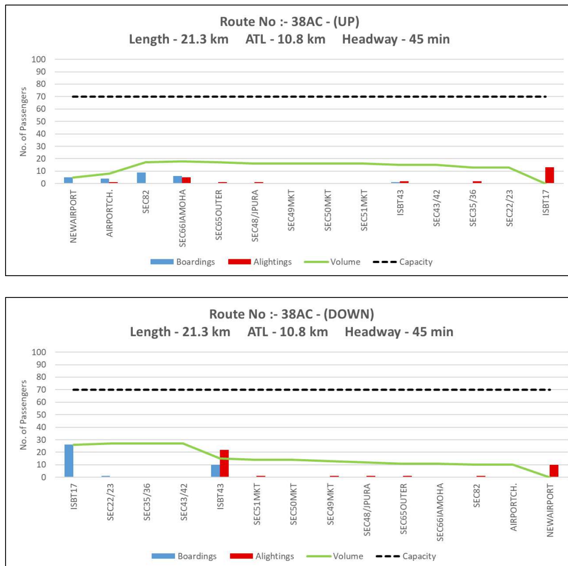
Figure 55: Peak hour Boarding & Alighting pattern along with line load of Route 38AC (Up and Down)
